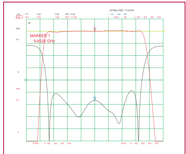
Passband Response
